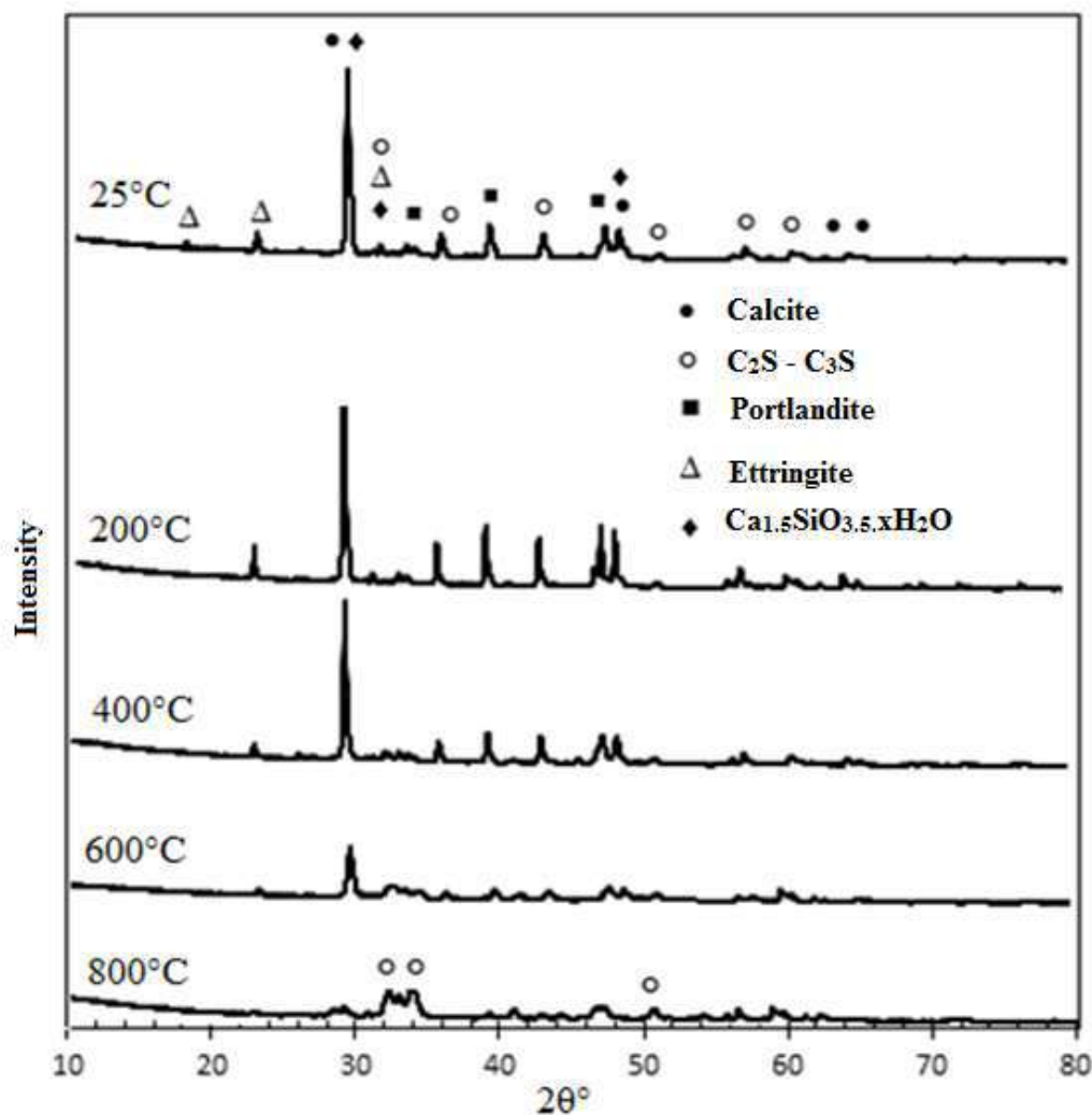
Figure 1. XRD Result of Cement Paste
