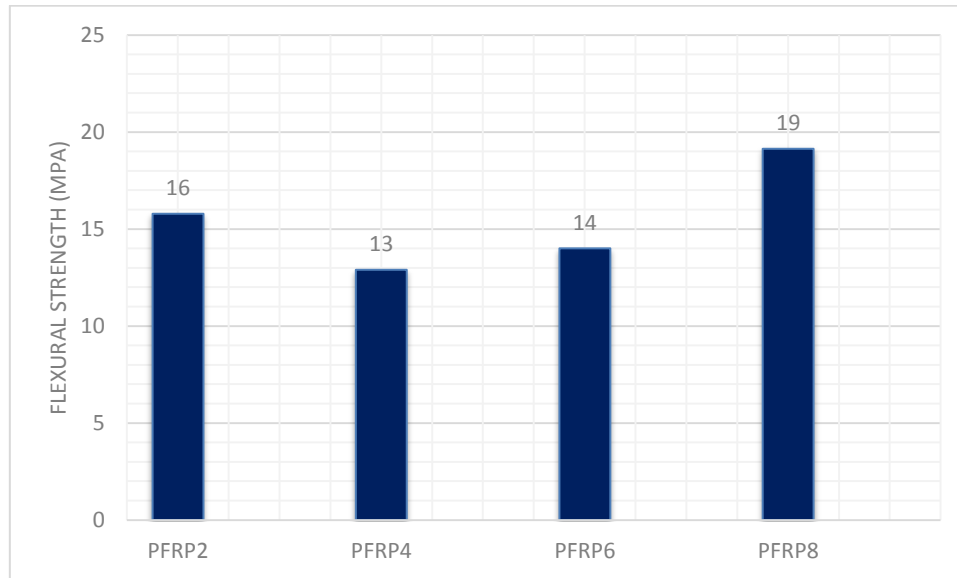
Figure 6 Flexural strength results
