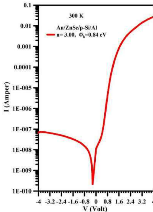
Figure.5. I-V characteristics graphs of Au/ZnSe/p-Si/Al device obtained from I-V measurements carried in dark and at room temperature.
