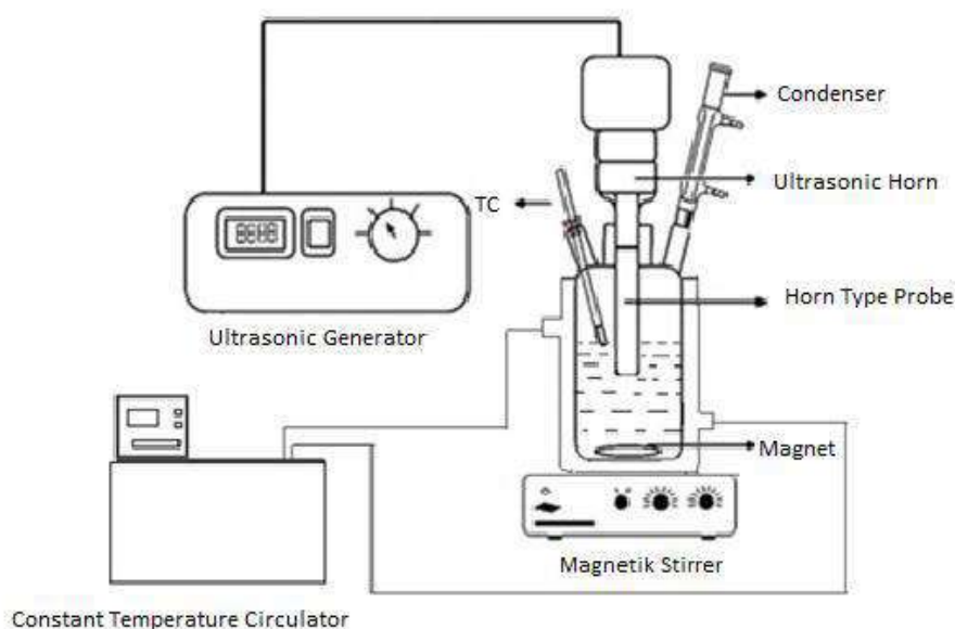
Figure 1. The set-up for ultrasonic experiments
