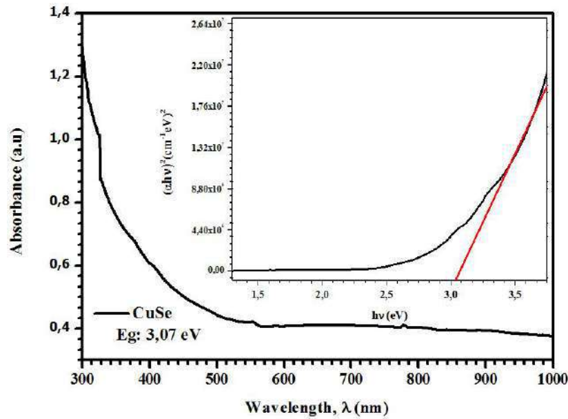
Figure 1. Variation of optical absorbance versus the wave-length of incident photons of the as-deposited and (\alpha h\nu)^2 versus h\nu plots (in small frames) corresponding to CuSe thin film.
