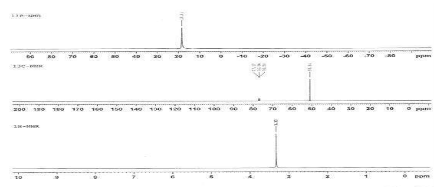
Figure 6. NMR spectrum of reference material
