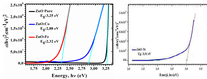
Fig.2. Shows the plot of (\alpha h\nu)^2 versus h\nu and transmittance spectra of films for ZnO, Co, Ni, Fe doped ZnO
