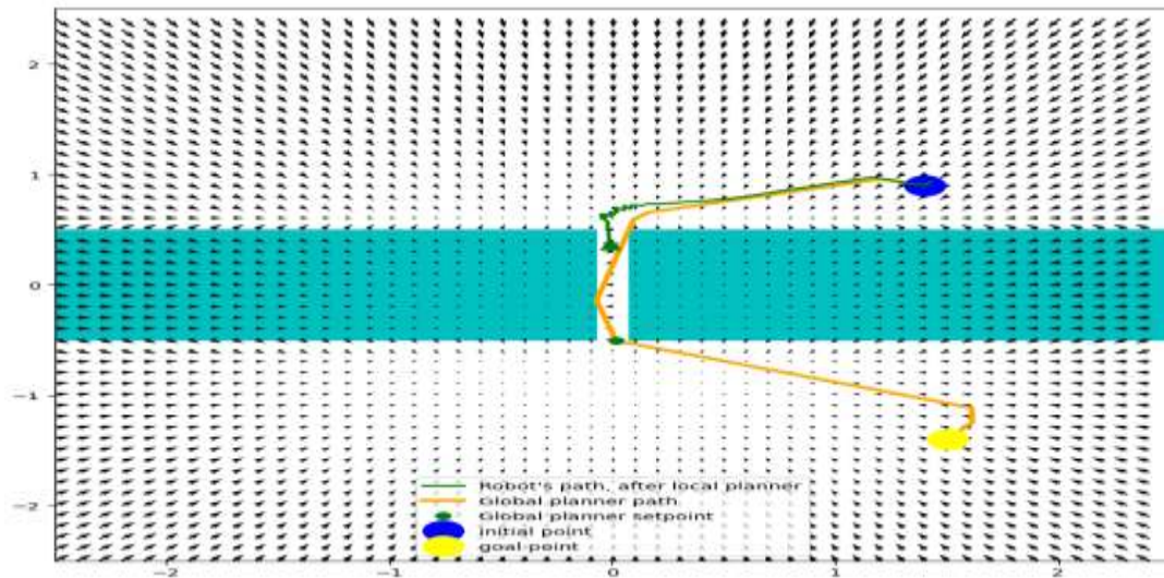
Fig. 7. Robot's Path After Local Planner Progress Output-1
