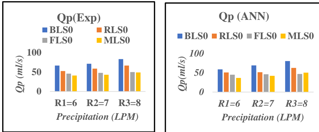
Fig. 4. (a) , (b) Peak flow (Experimental and ANN) values for all cases at 0° slope.
